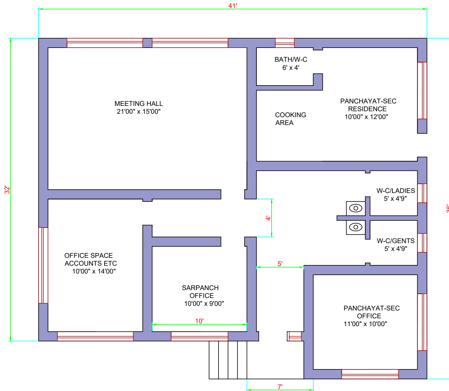
BUILDING PLAN OF PANCHAYAT GHAR WITH BOTH MEETING HALL AND RESIDENTIAL ACCOMMODATION FOR PANCHAYAT SECRETORY.
