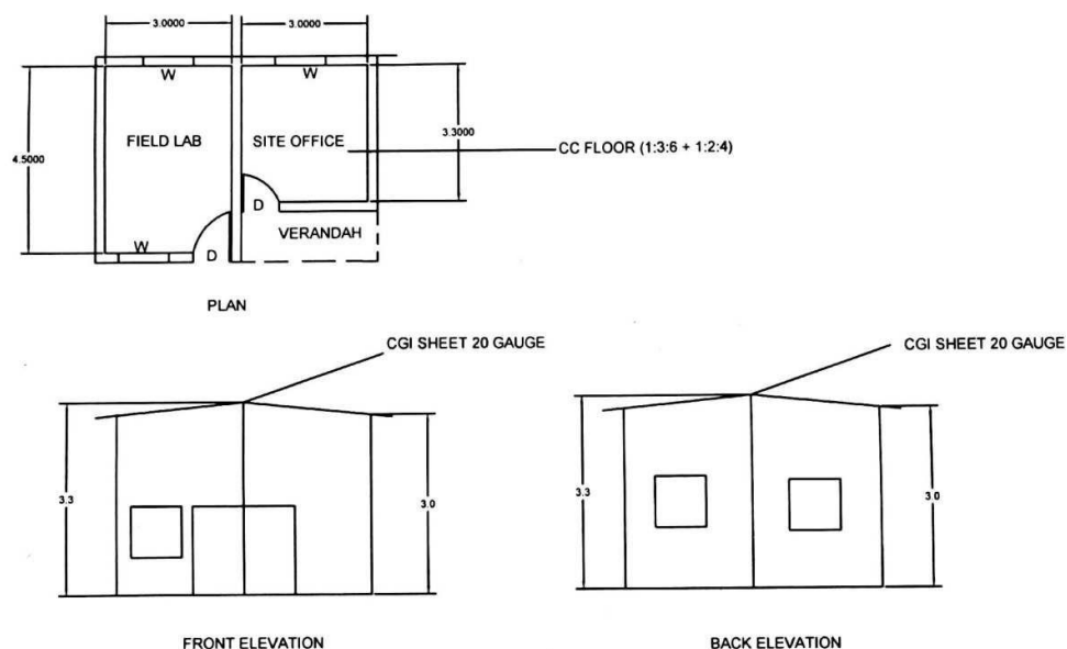
Schematic Diagram for Field Laboratory and Site Office
