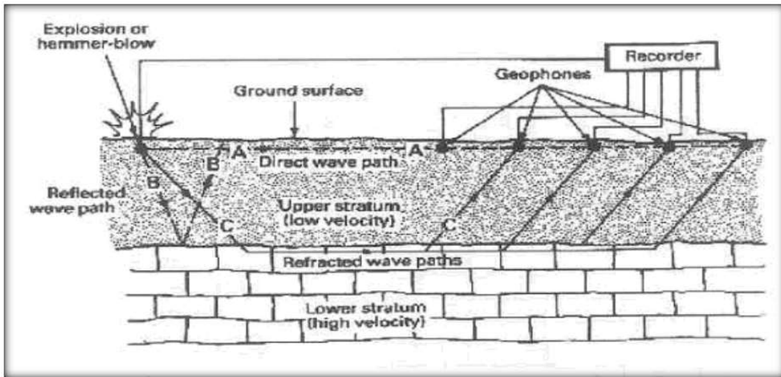
Fig. - 2 : Principle of Seismic Refraction Survey
