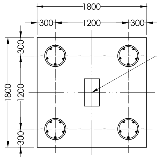
LAYOUT PLAN OF PC3 R.C.C. DETAILS OF 4 PILES GROUP CAPS (PC2)
