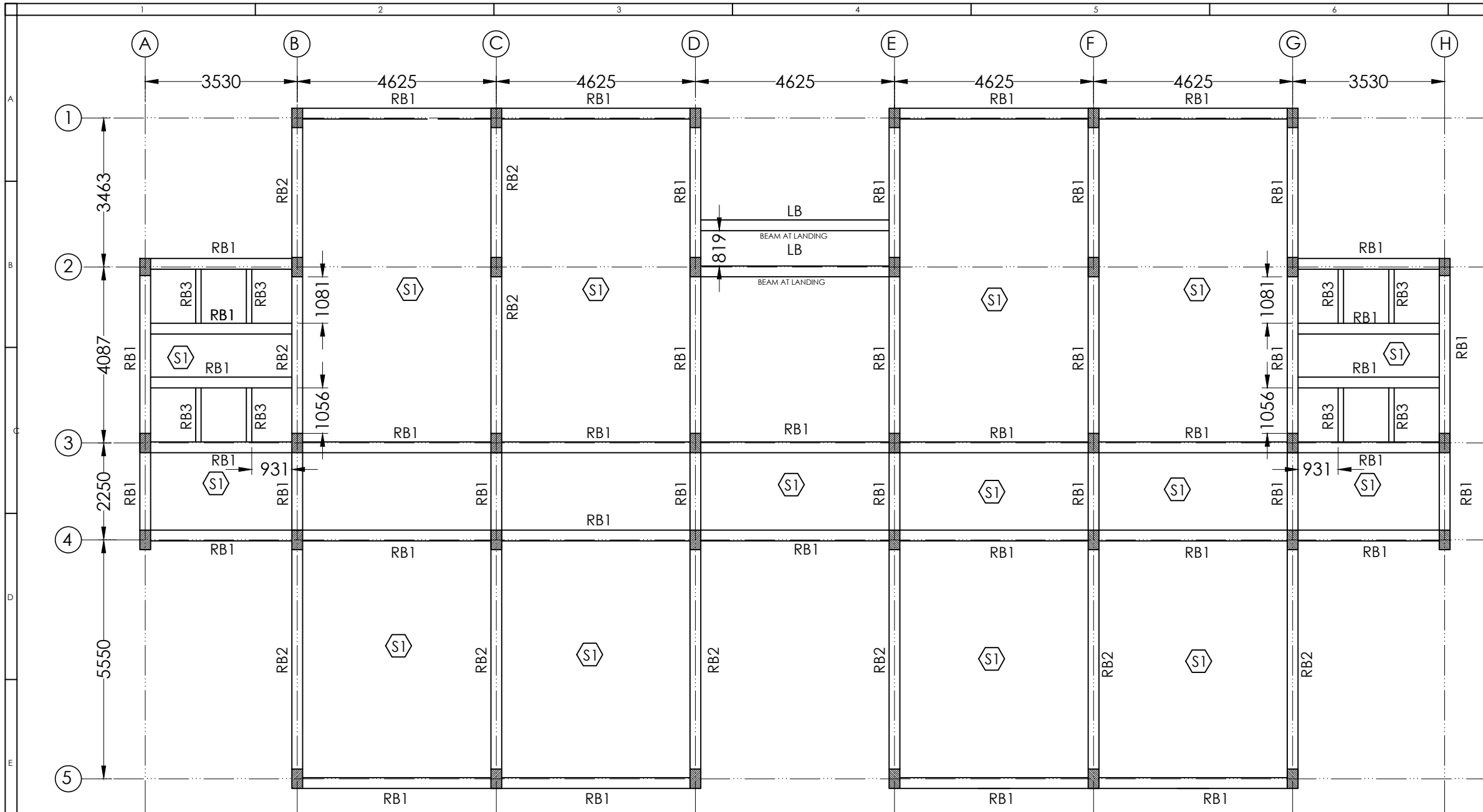
FIRST FLOOR ROOF BEAM LAYOUT PLAN
