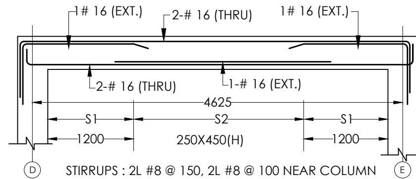
DETAILS OF LB
