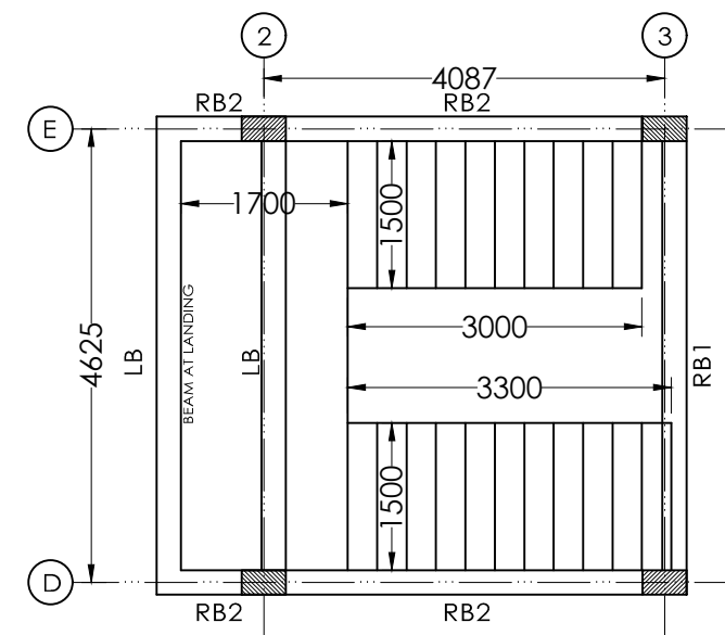
LAYOUT PLAN OF STAIRCASE AT ±0.60M LVL.
