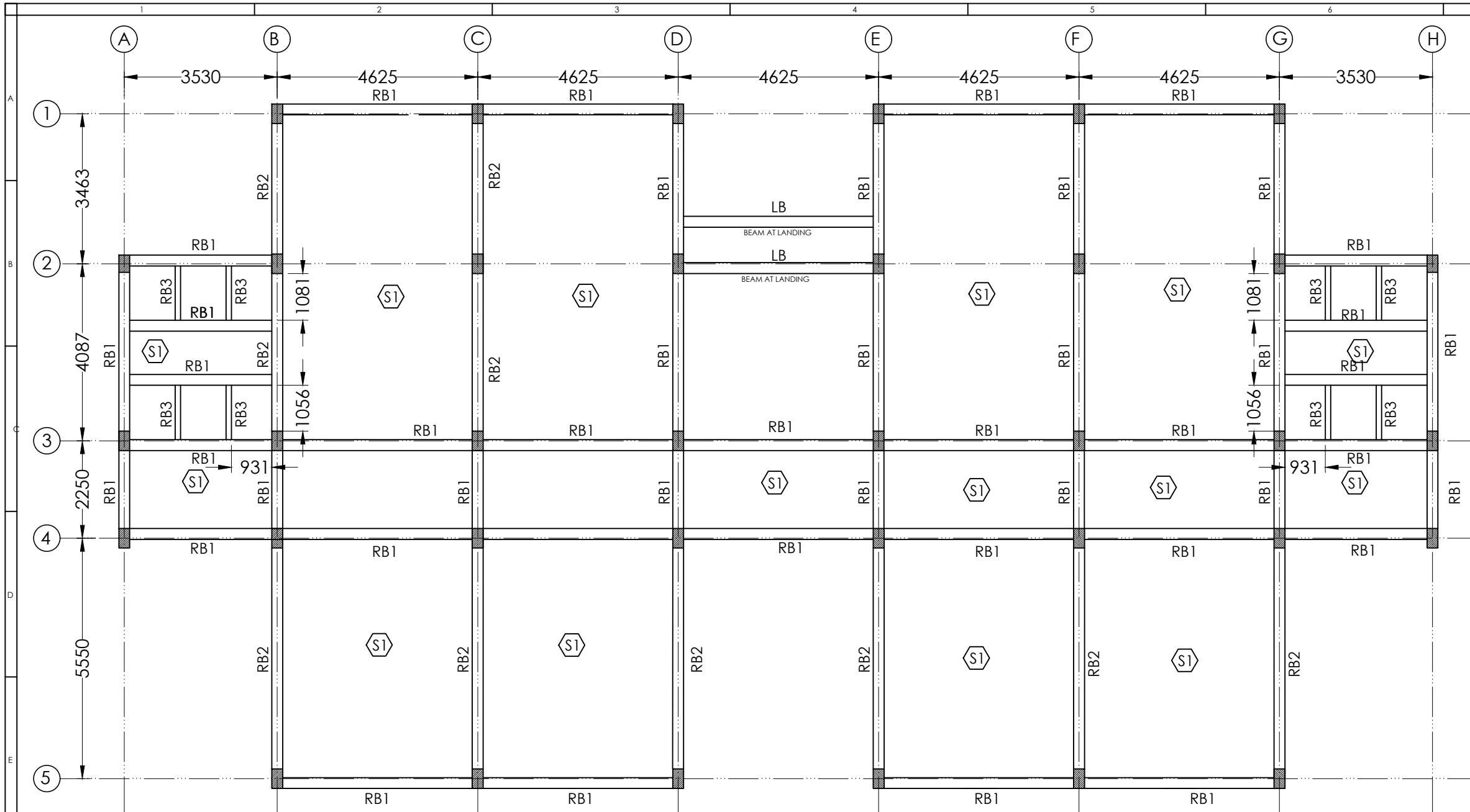
SECOND FLOOR ROOF BEAM LAYOUT PLAN
