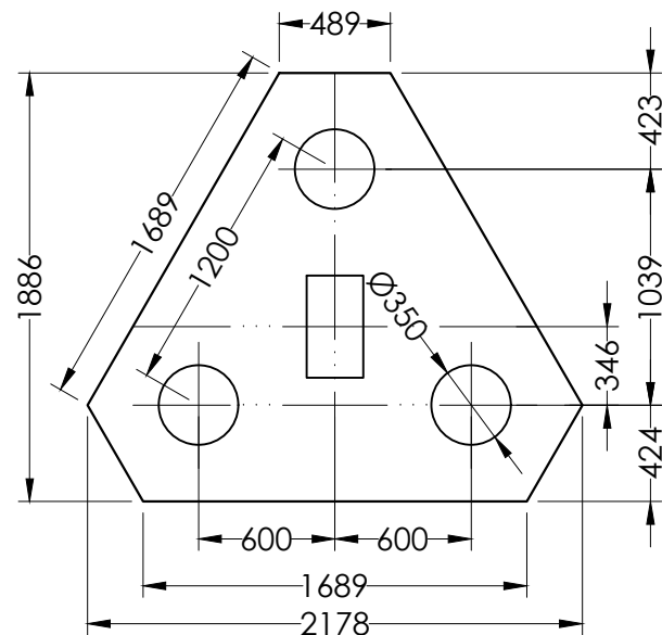
LAYOUT PLAN OF PC1 R.C.C. DETAILS OF 3 PILES GROUPCAPS (PC1)
