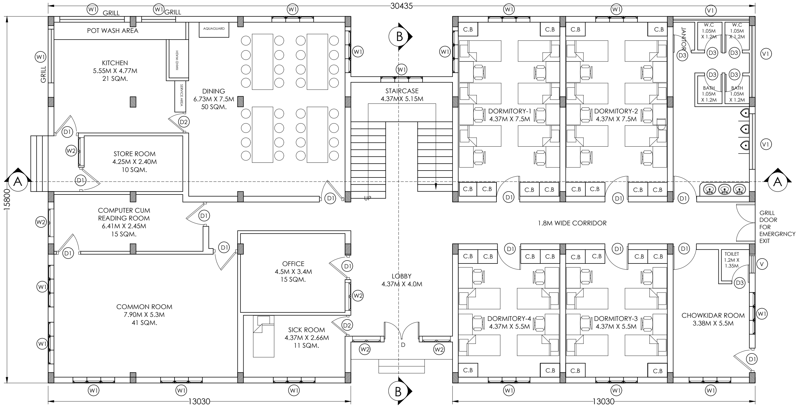
GROUND FLOOR PLAN 461 SQM
