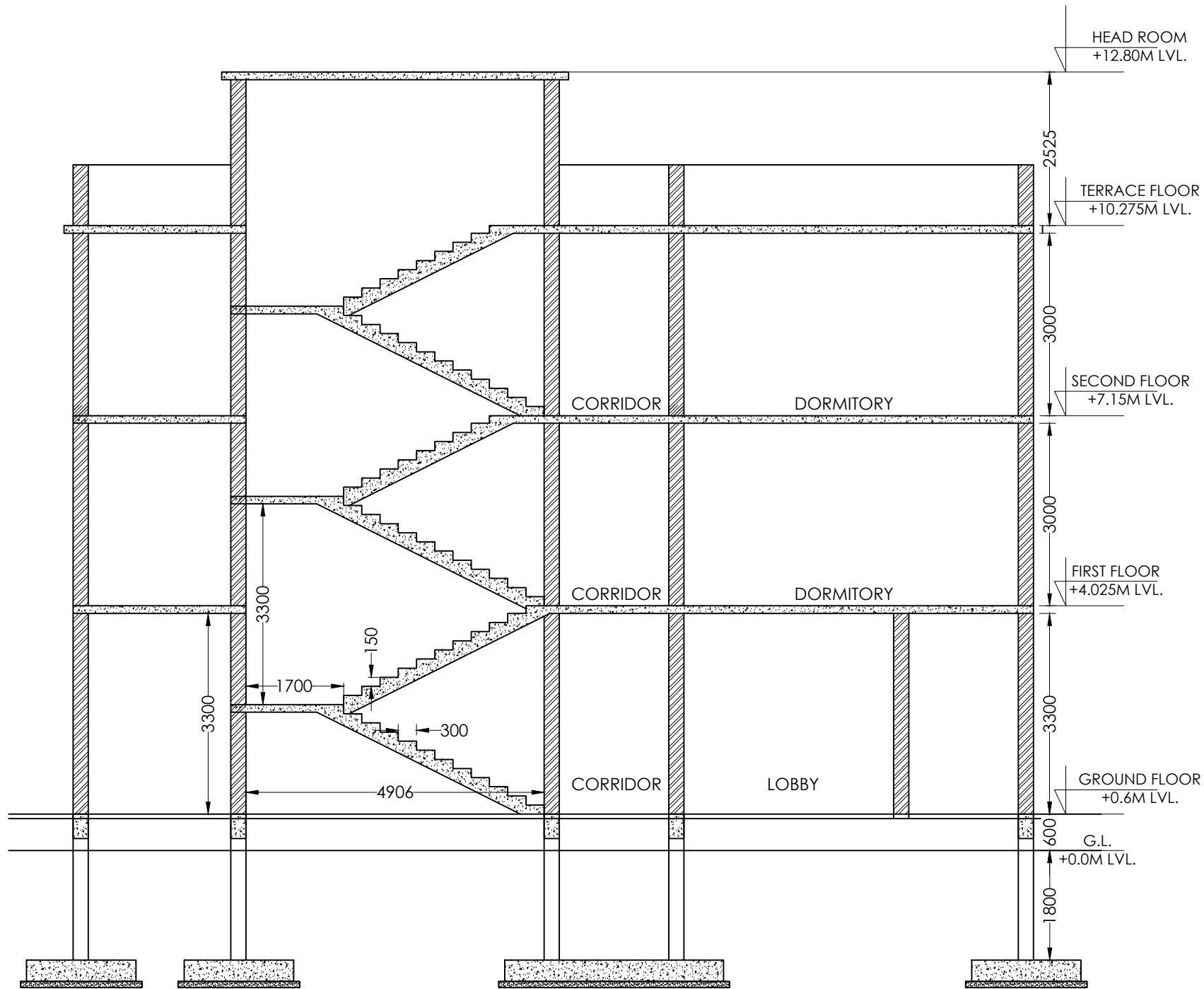
SECTION- BB
