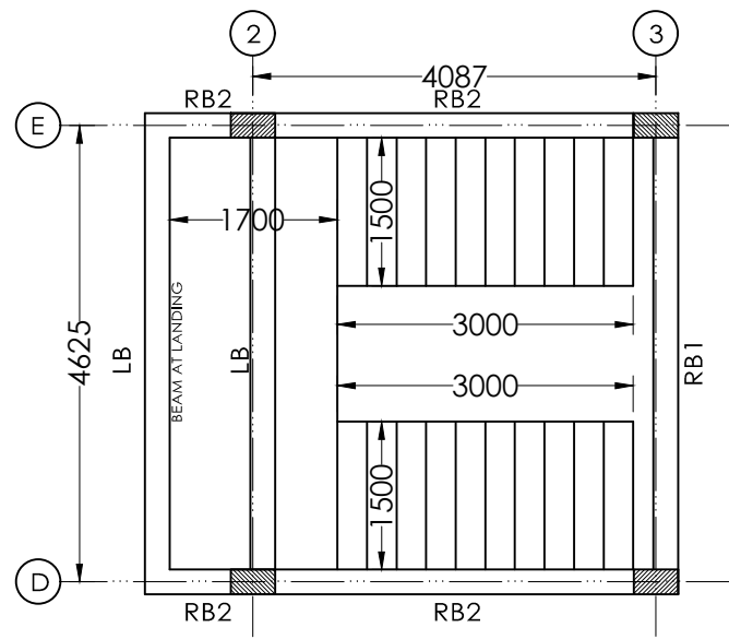
LAYOUT PLAN OF STAIRCASE AT ±4.025M LVL.
