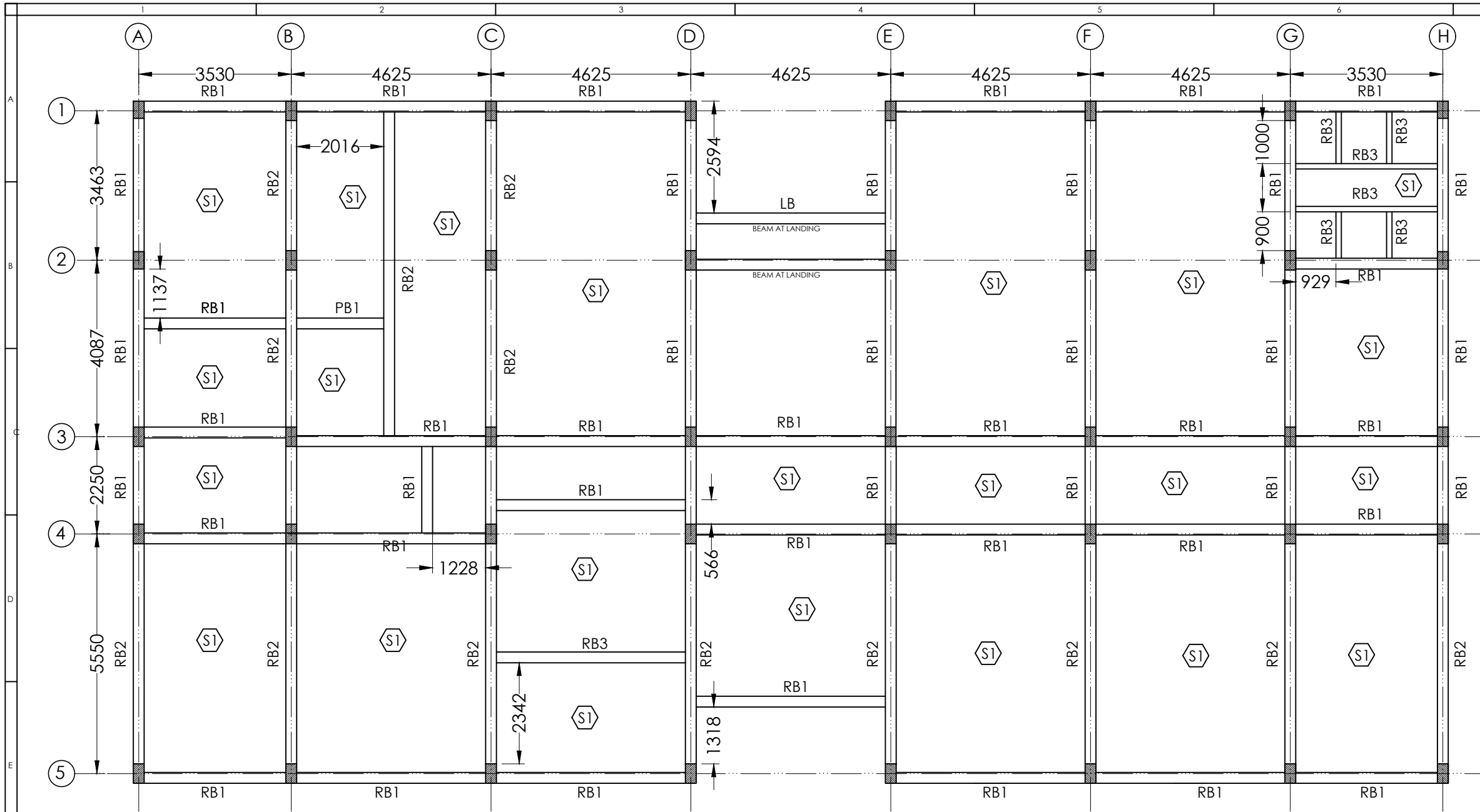
GROUND FLOOR ROOF BEAM LAYOUT PLAN
