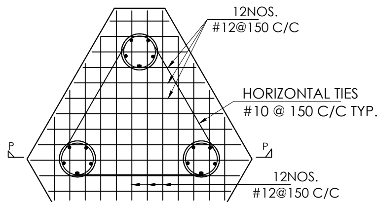
PLAN OF BOTTOM STEEL
