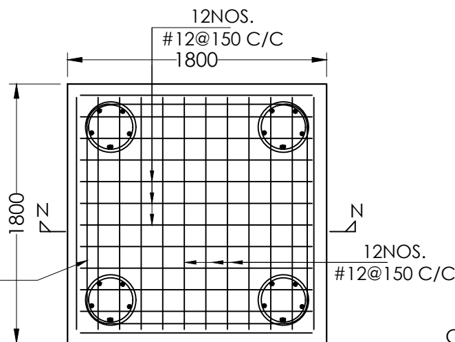
PLAN OF BOTTOM STEEL
