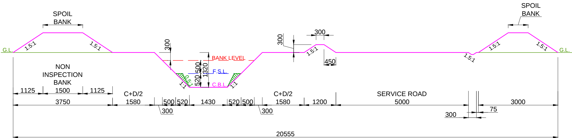
DESIGN SECTION FROM CH: 0.000 KM TO CH: 0.450 KM
