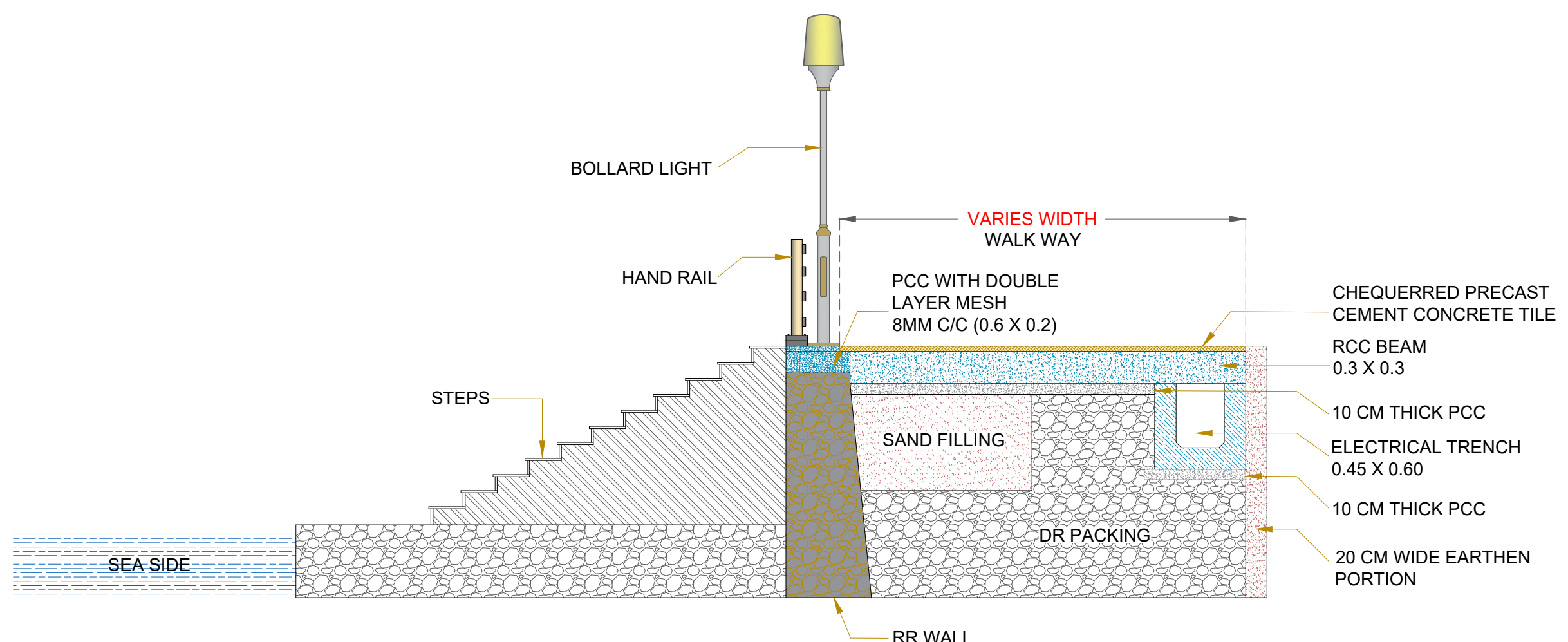
TIPYCAL CROSS SECTION-AA
