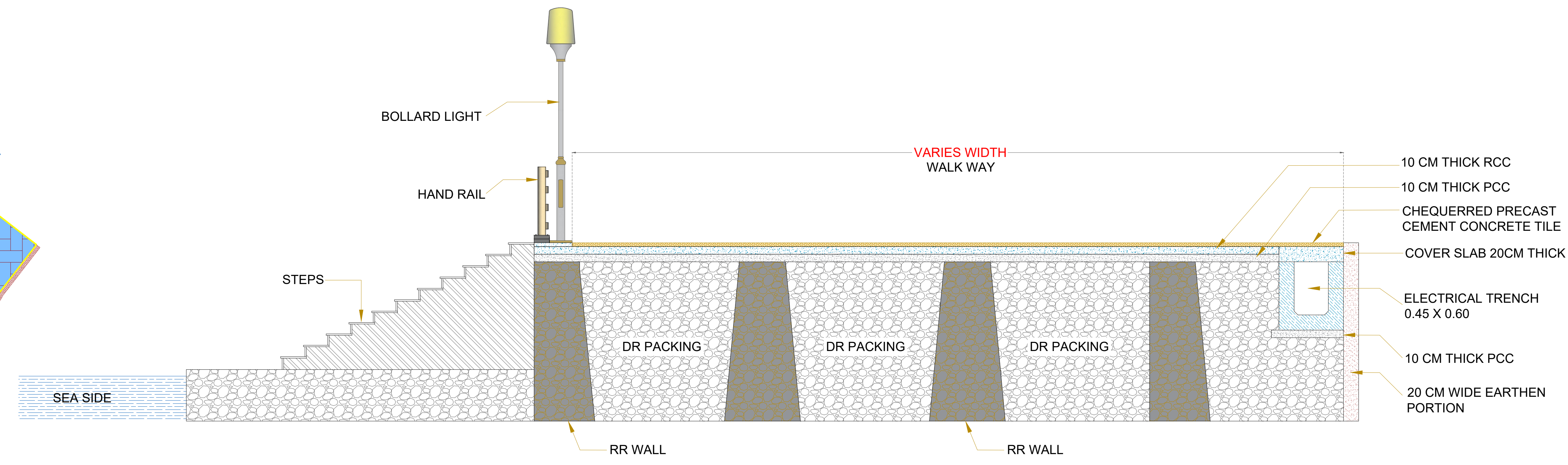
TIPYCAL CROSS SECTION-AA
