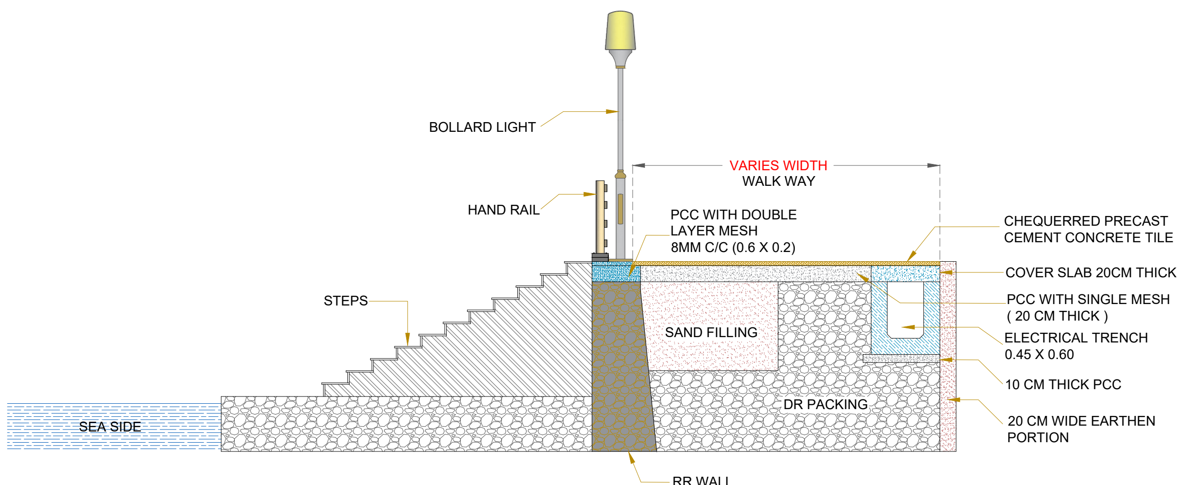
TIPYCAL CROSS SECTION-BB
