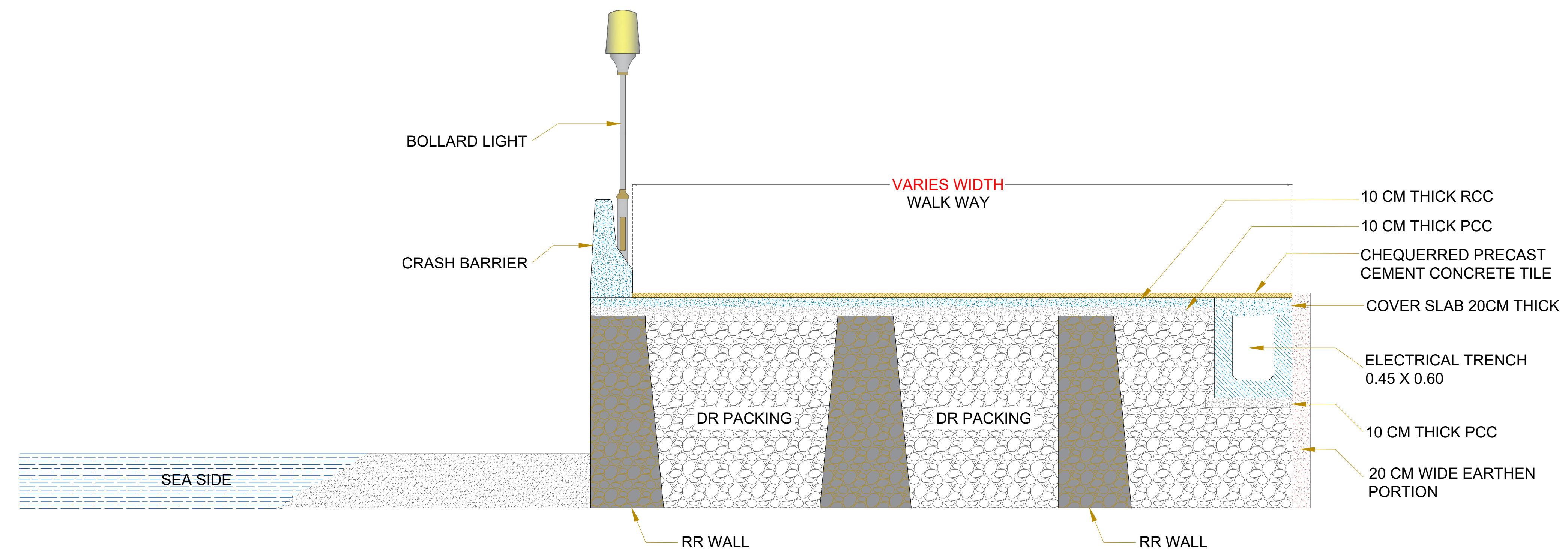
TIPYCAL CROSS SECTION-BB
