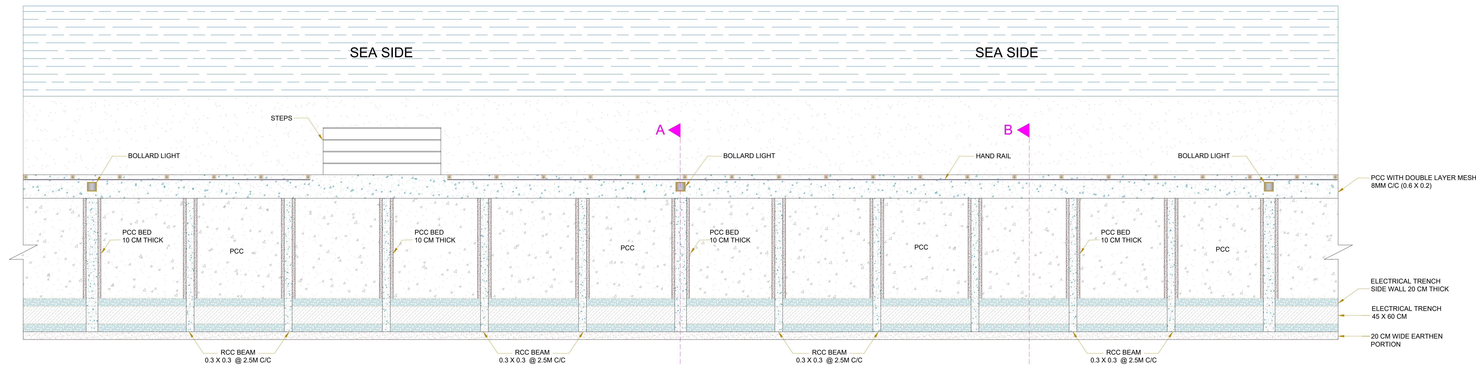
PLAN
