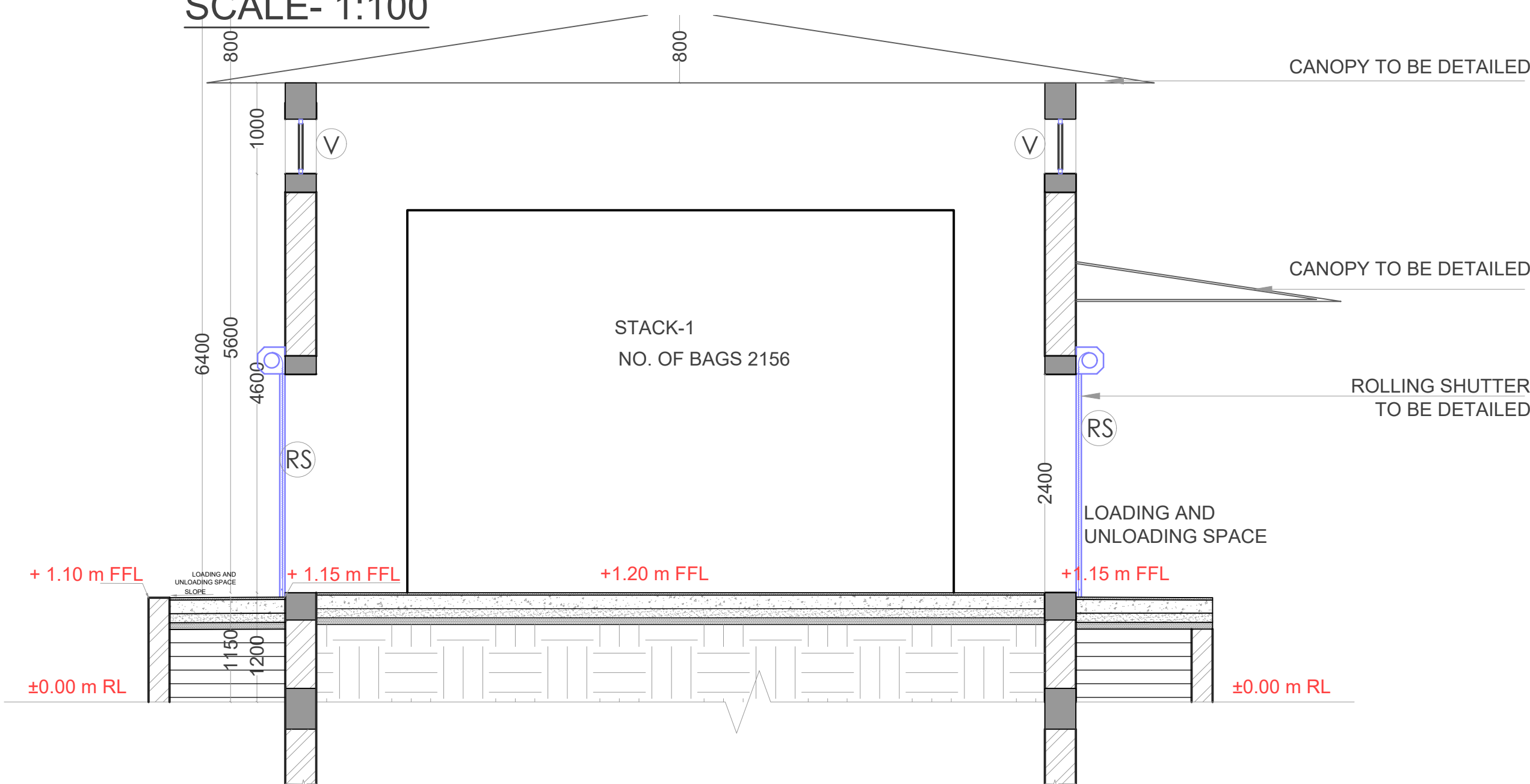
SECTION-BB SCALE- 1:100
