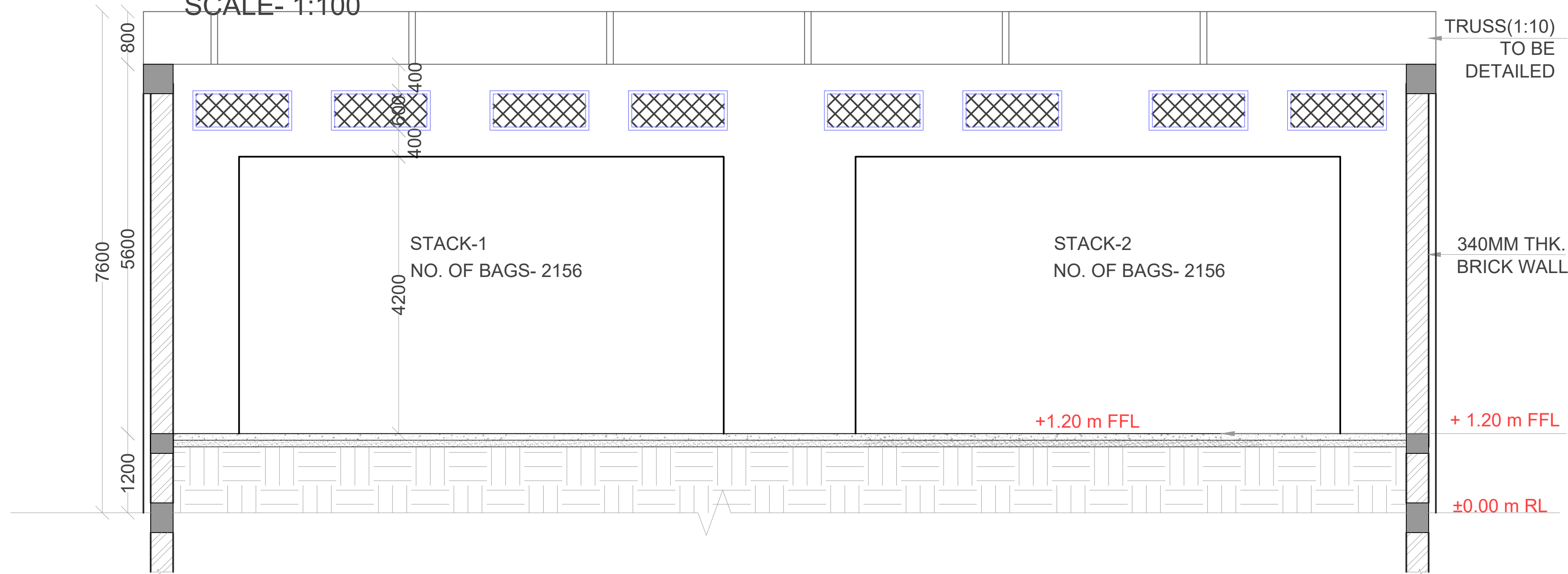
SECTION-AA SCALE- 1:100
