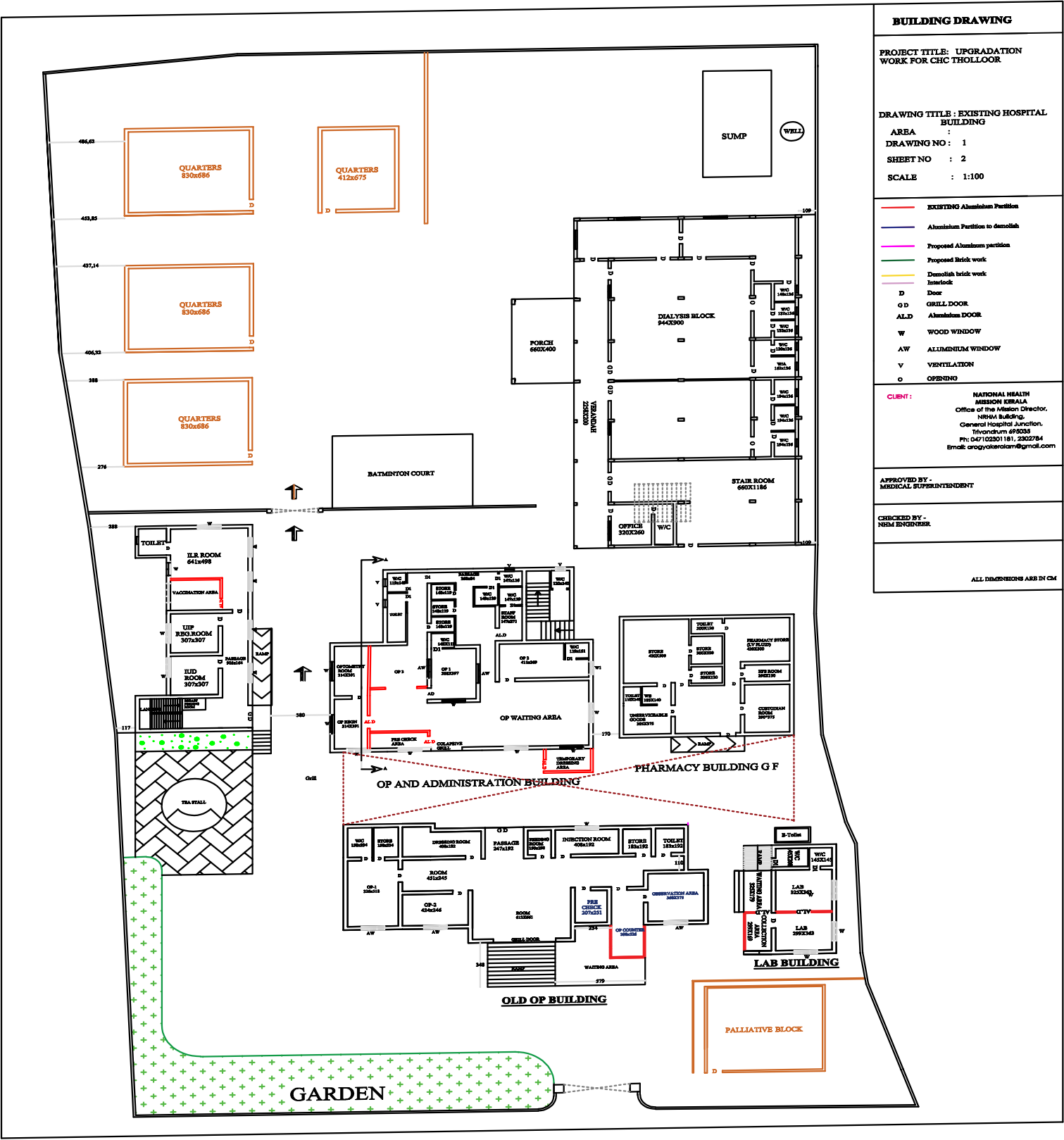
EXISTING DRAWING
