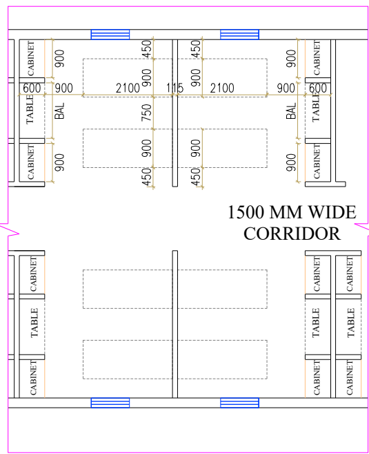
TYPICAL FURNITURE LAYOUT
