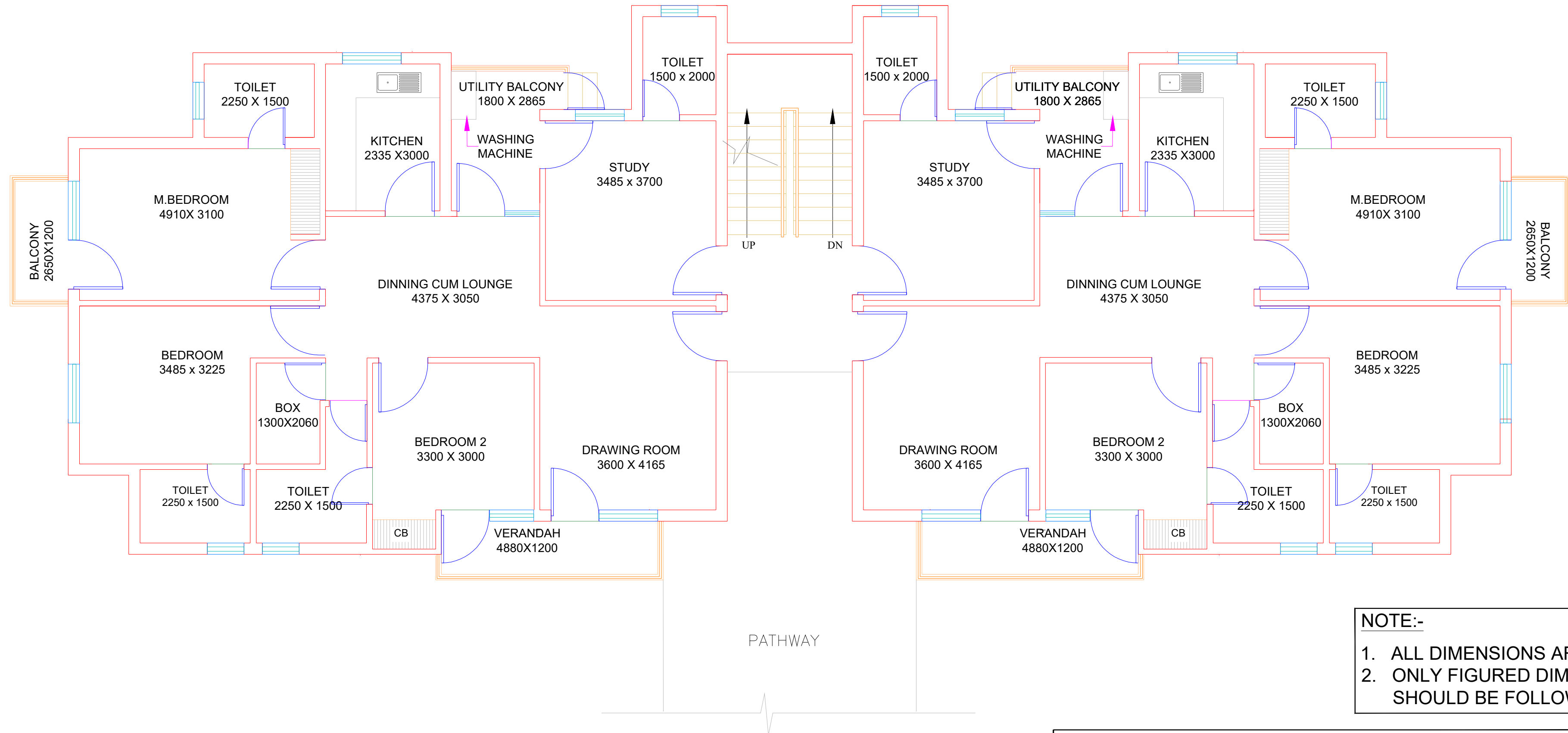
TYPICAL FLOOR PLAN G+3
