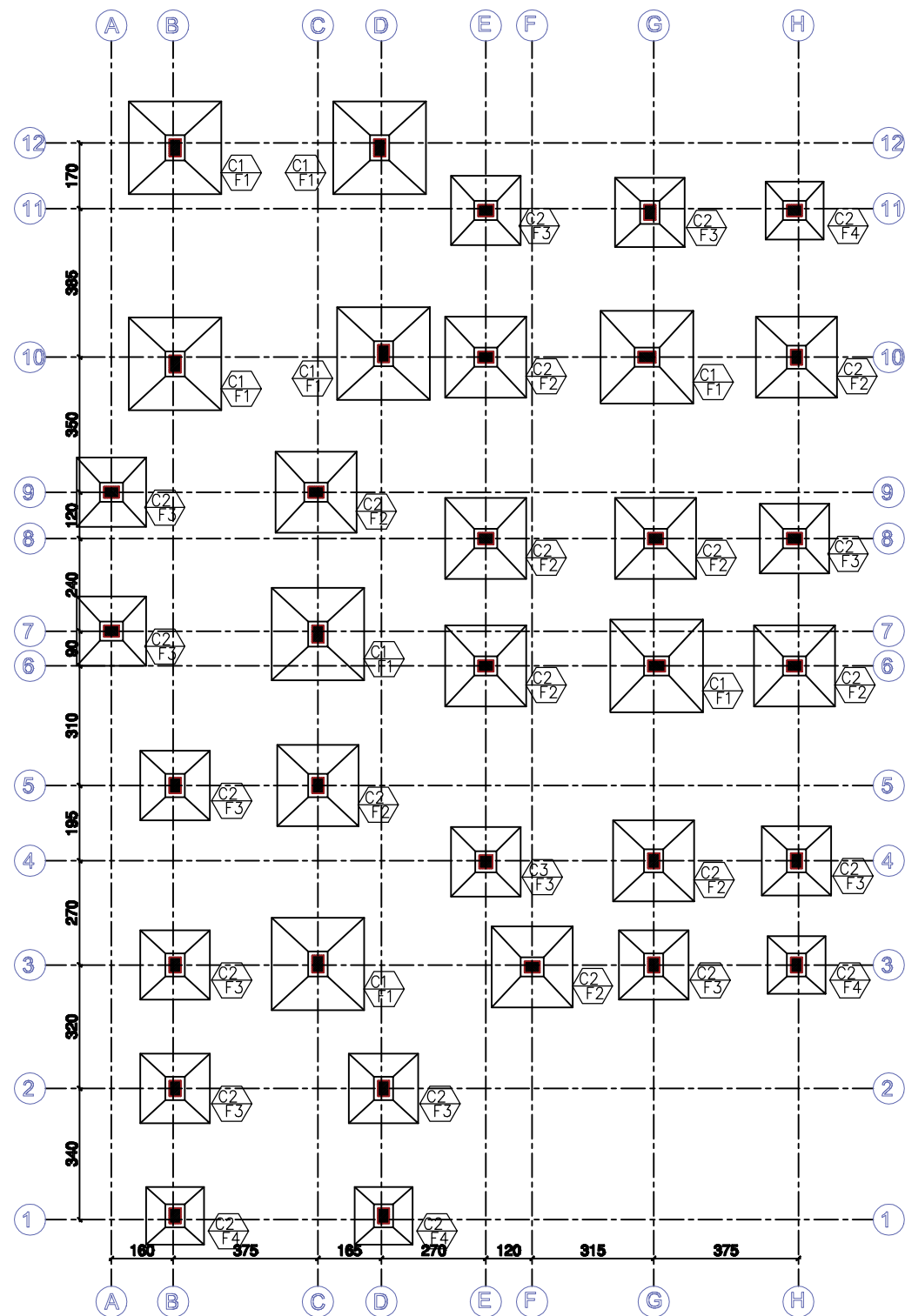
COLUMN & FOOTING LAYOUT
