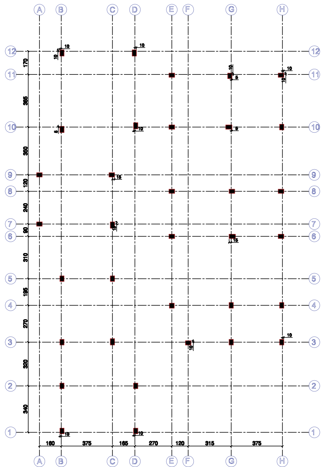
COLUMN MARKING LAYOUT
