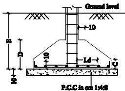
FOOTING SECTION
