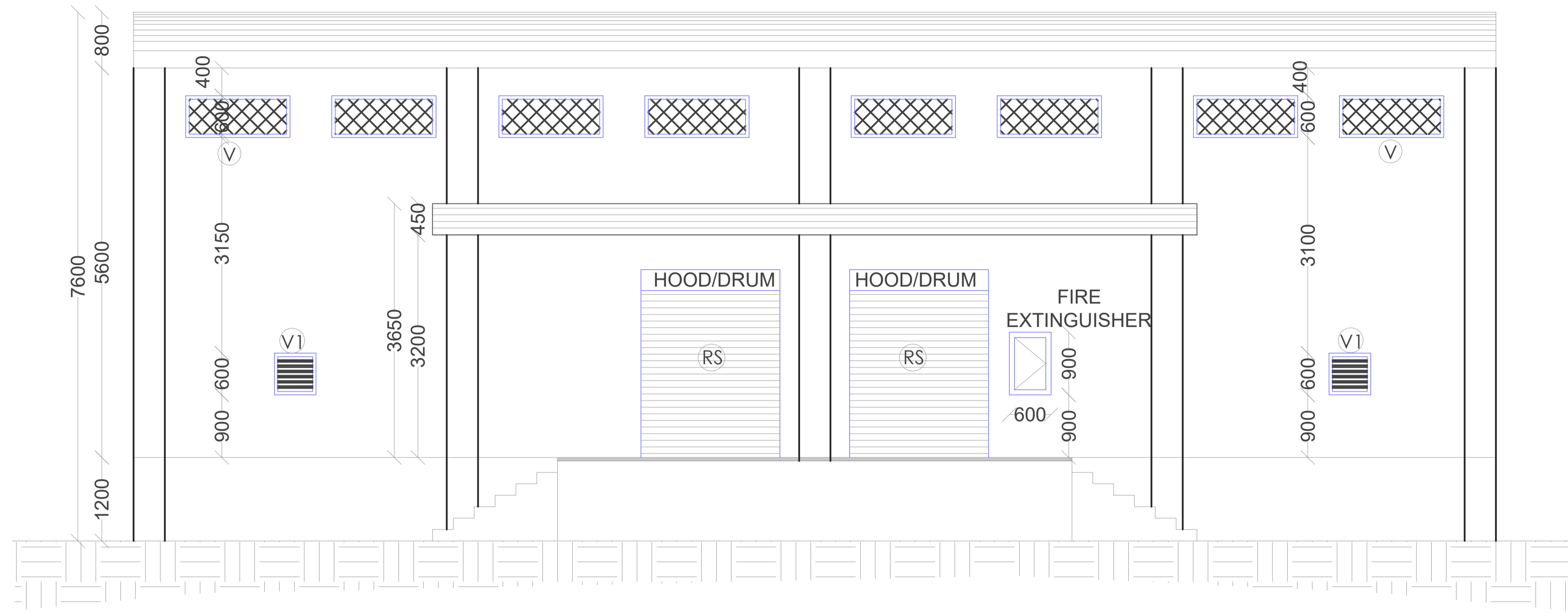
ELEVATION SCALE- 1:100
