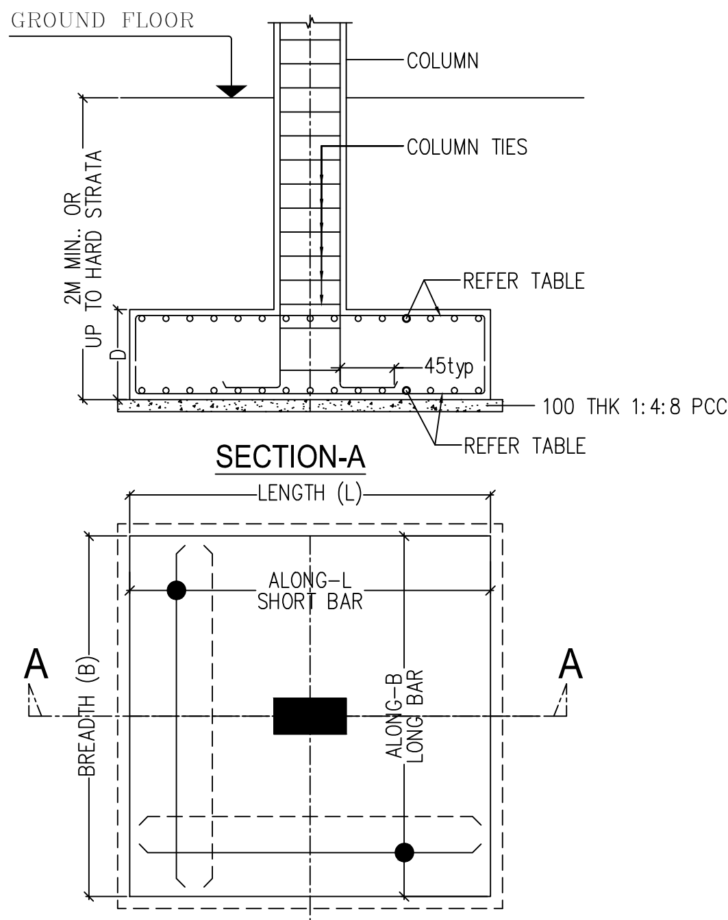
TYPICAL ISOLATED FOOTING
