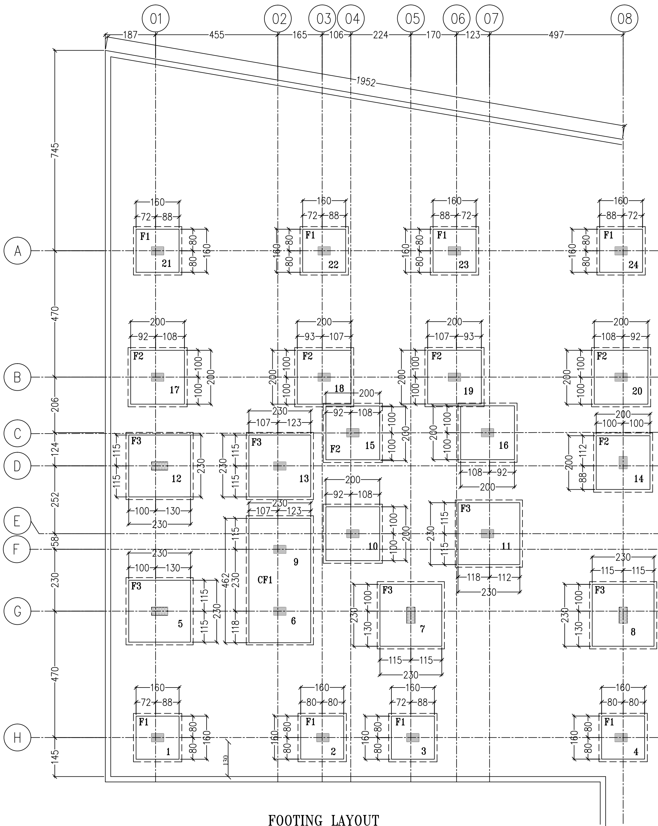
FOOTING LAYOUT
