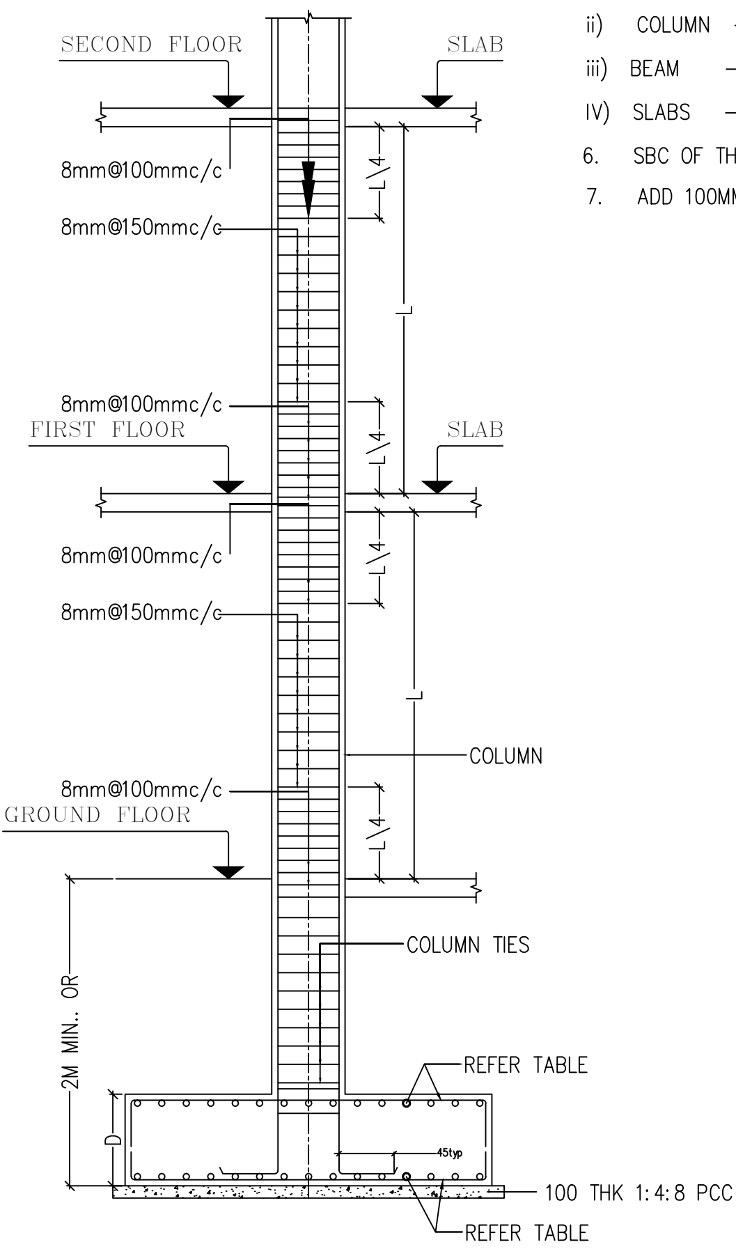
TYPICAL LATERAL TIES ARRANGEMENT FOR COLUMNS
