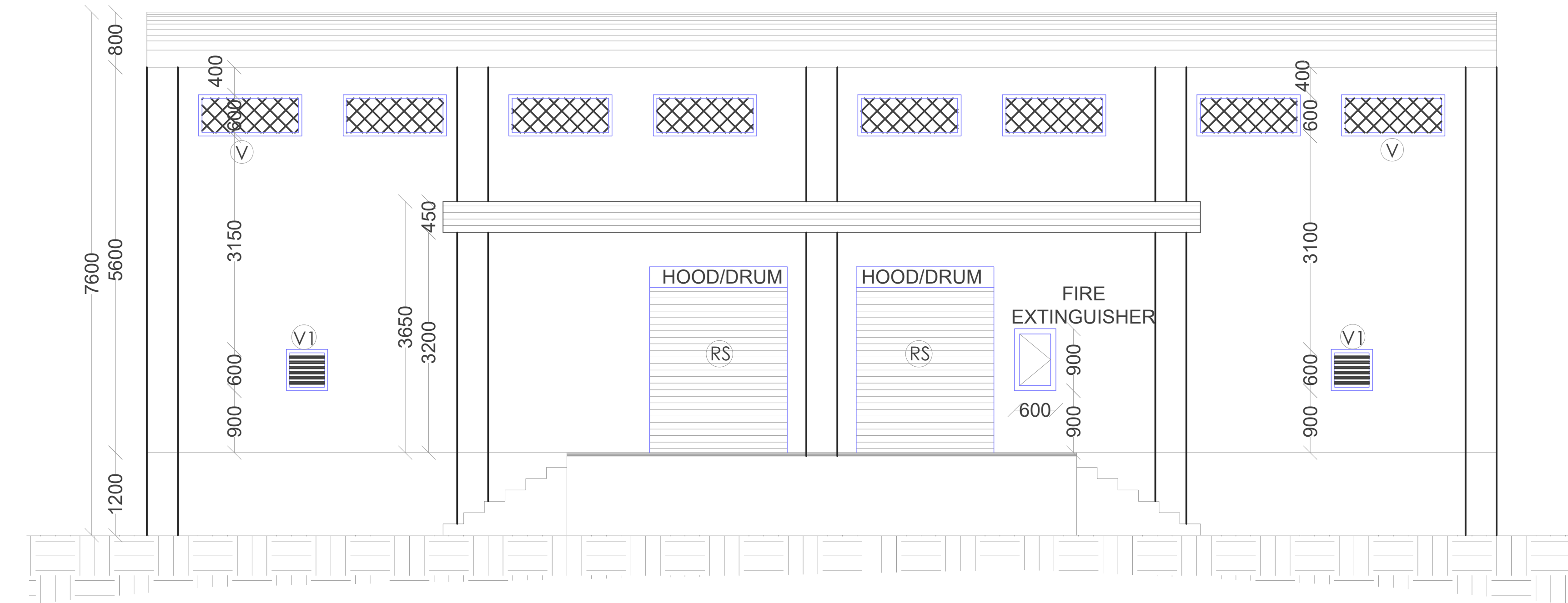
ELEVATION SCALE- 1:100
