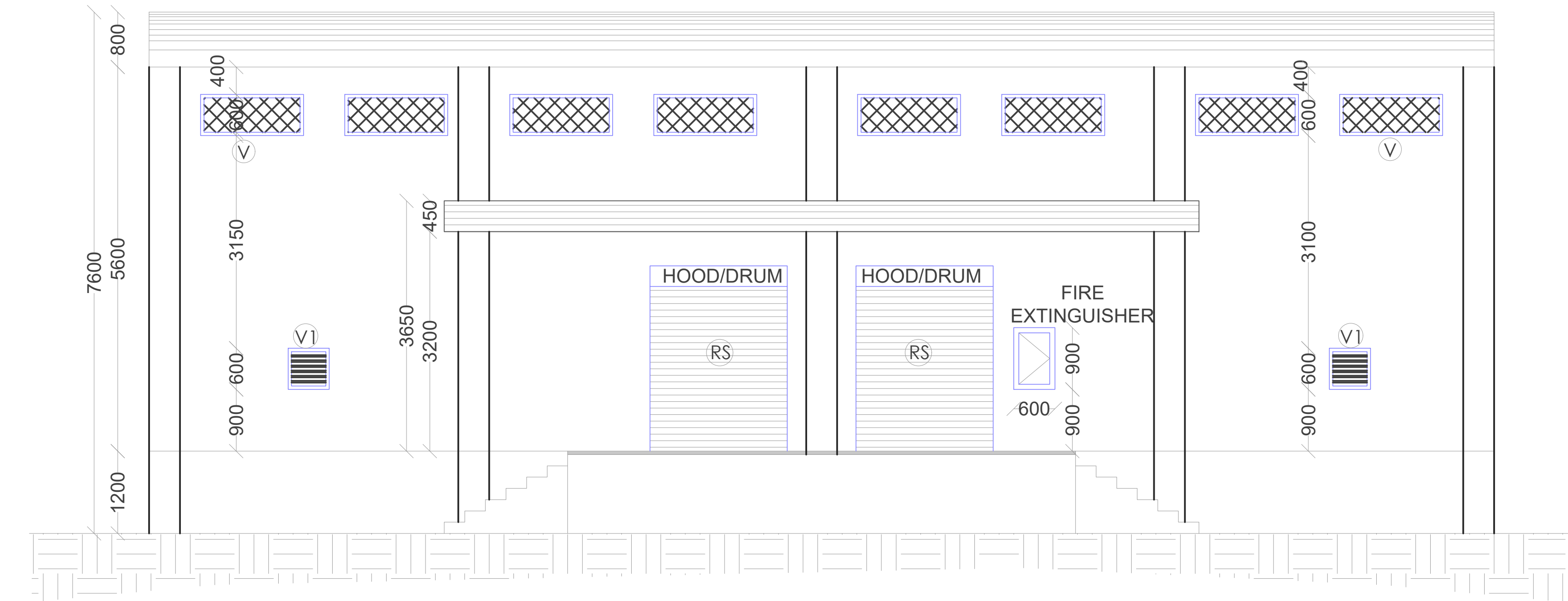
ELEVATION SCALE- 1:100
