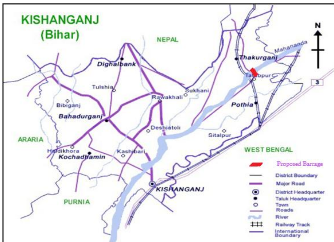
Figure 1.1: Proposed Barrage on Mahananda River at Taiyabpur
