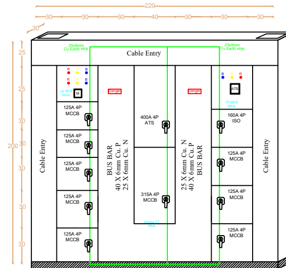
FRONT VIEW OF (One Panel) MSB W&C
