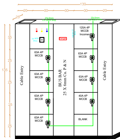
FRONT VIEW OF (5Nos Panel) SSB GF, FF, SF, TF & EQ
