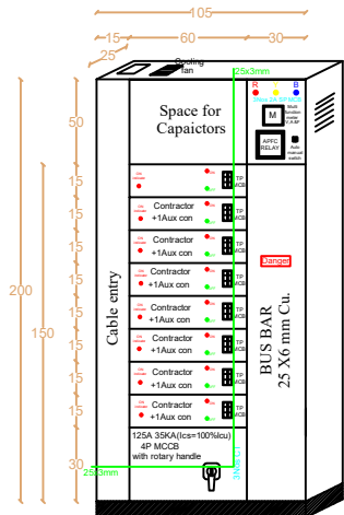
FRONT VIEW OF (One Panel) APFC Panel
