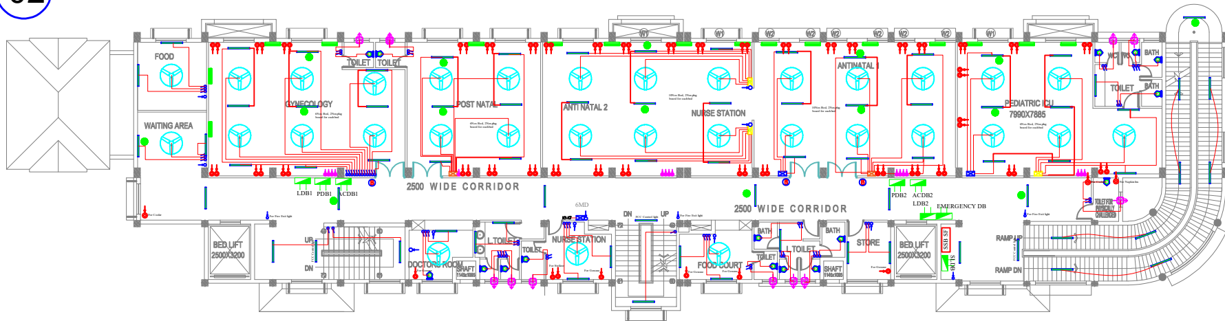
SECOND FLOOR
