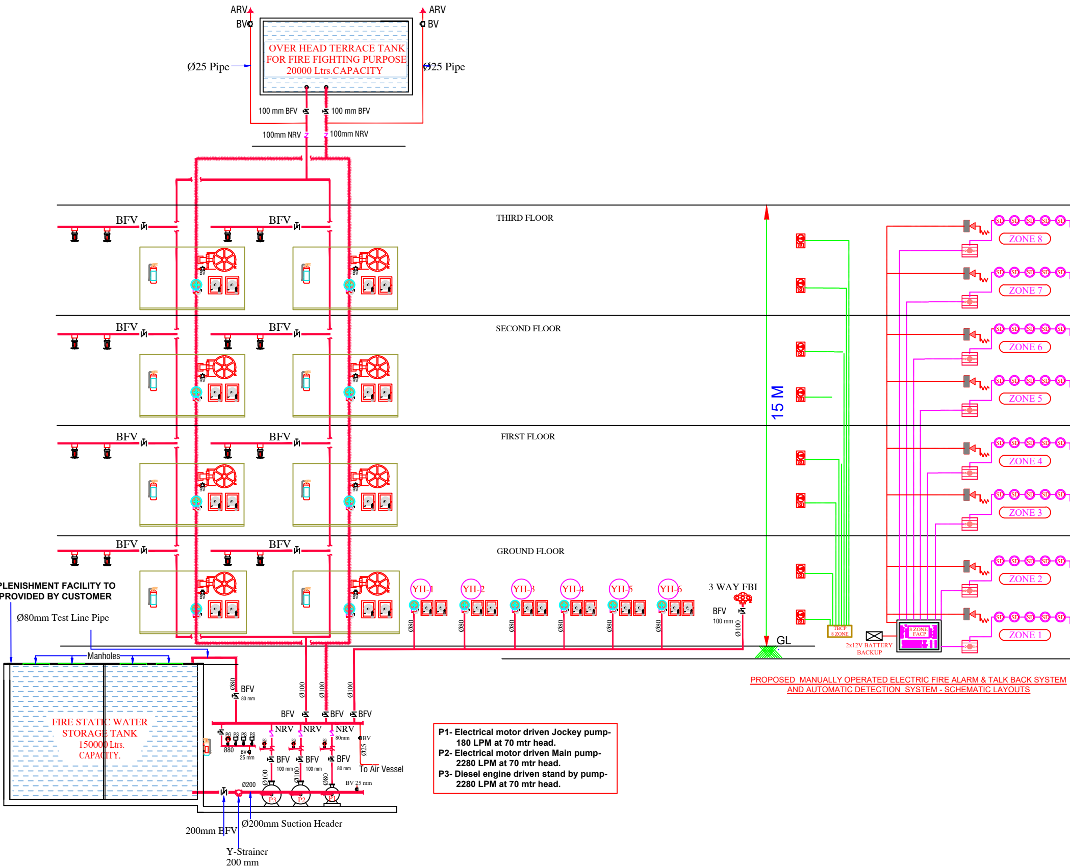
PROPOSED FIRE PROTECTION SYSTEM -SCHEMATIC LAYOUT (WET RISER SYSTEM)
