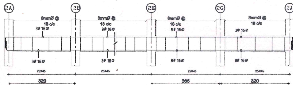
BEAM PB6 (2A-2J)
