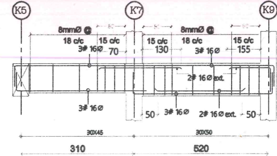
BEAM FB13A (K5-K9)
