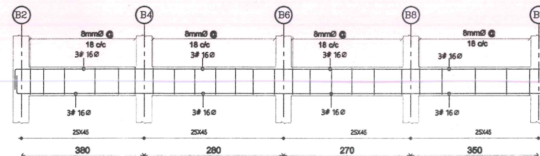
BEAM PB9 (B2-B9)
