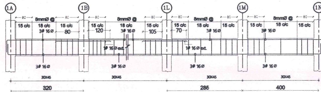
BEAM FB7 (1A-1N)
