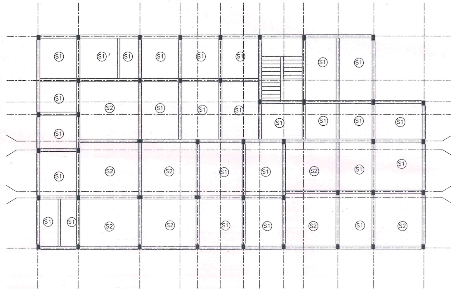
FLOOR SLAB LAYOUT
