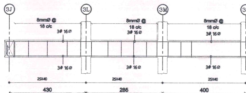
BEAM PB5 (3J-3N)
