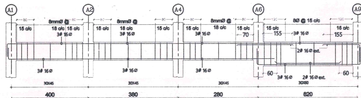
BEAM FB8 (A1-A9)
