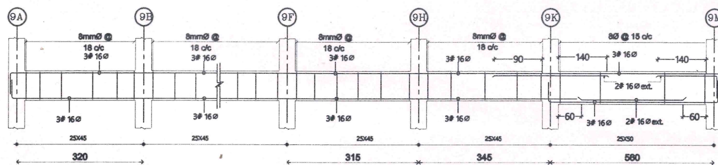
BEAM PB1 (9A-9M)
