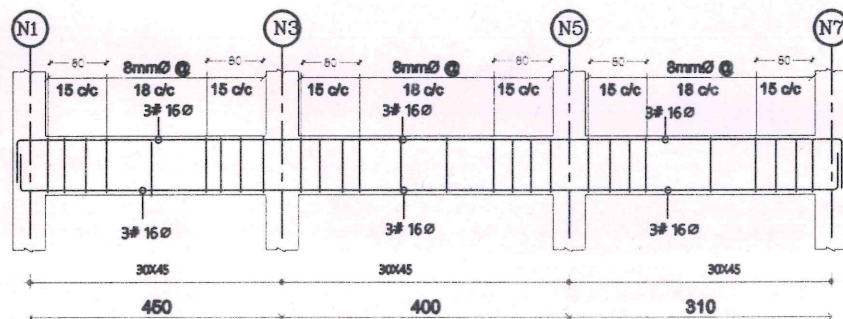
BEAM FB16 (N1-N7)
