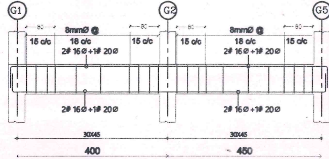
BEAM FB12A (G1-G5)
