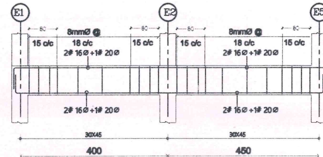
BEAM FB12 (E1-E5)
