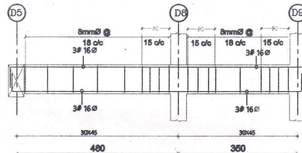
BEAM FB11 (D5-D9)
