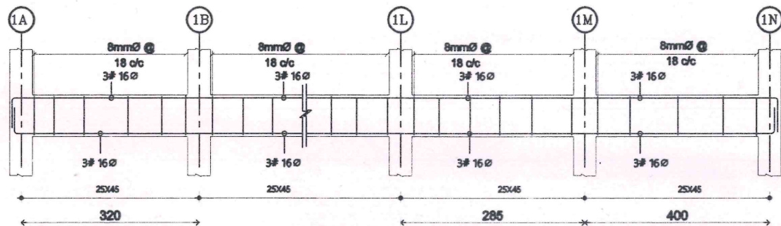
BEAM PB7 (1A-1N)
