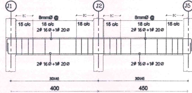
BEAM FB12B (J1-J5)
