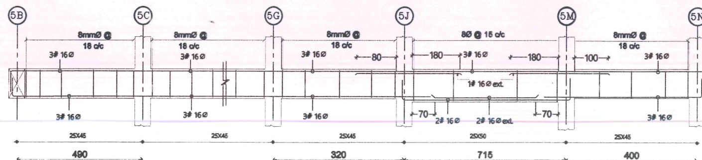
BEAM PB4 (5B-5N)
