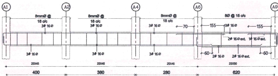
BEAM PB8 (A1-A9)
