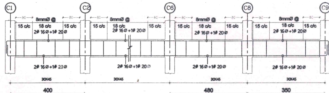
BEAM FB10 (C1-C9)
