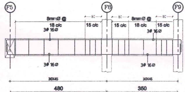
BEAM FB11A (F5-F9)
