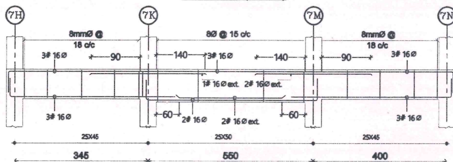
BEAM PB3 (7H-7N)
