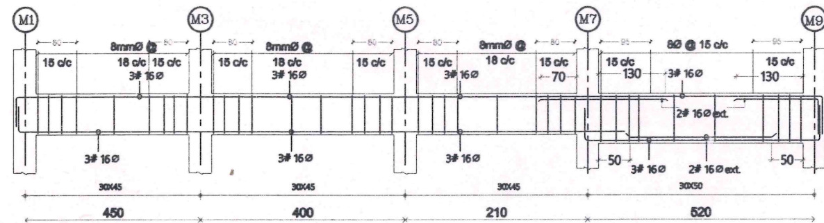
BEAM FB15 (M1-M9)
