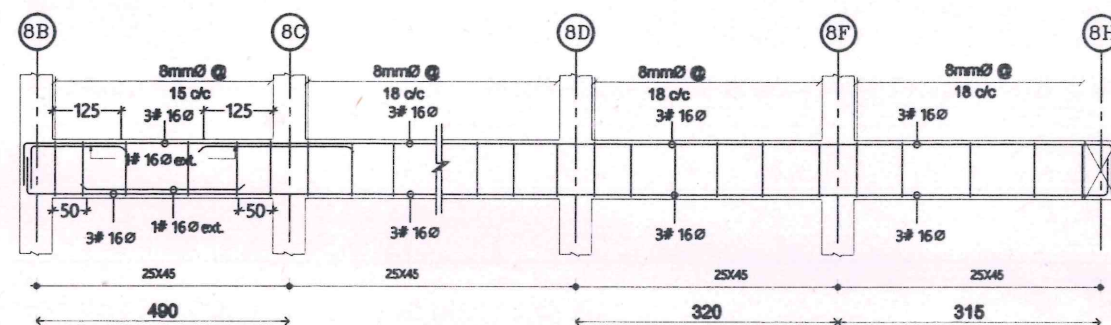
BEAM PB2 (8B-8H)
