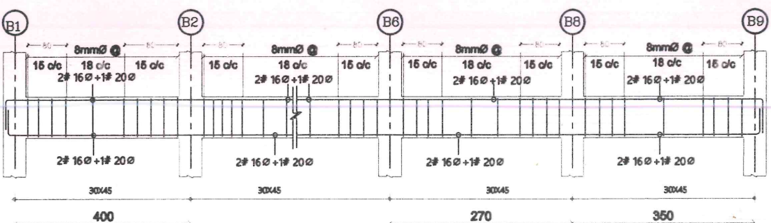
BEAM FB9 (B1-B9)
