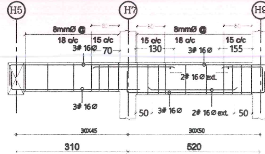
BEAM FB13 (H5-H9)
