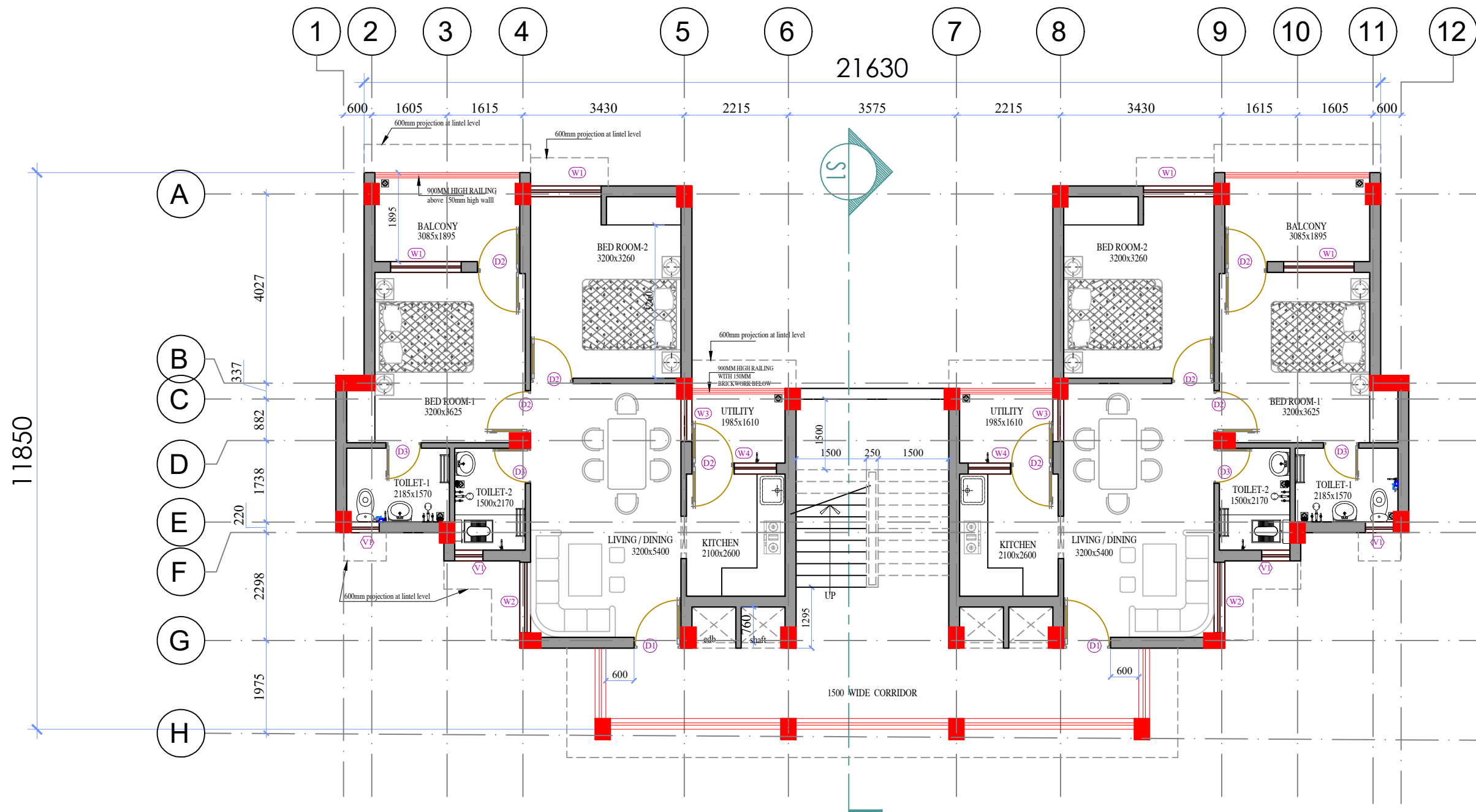
TYPICAL FLOOR PLAN.
