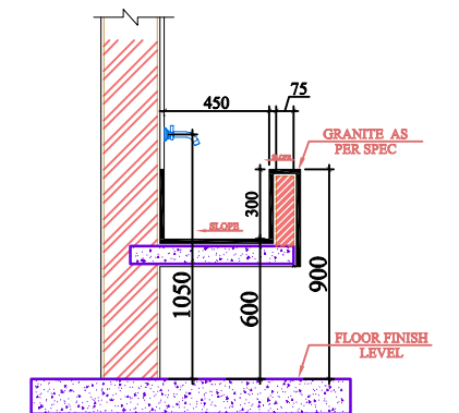
TROUGH TYPICAL SECTION
