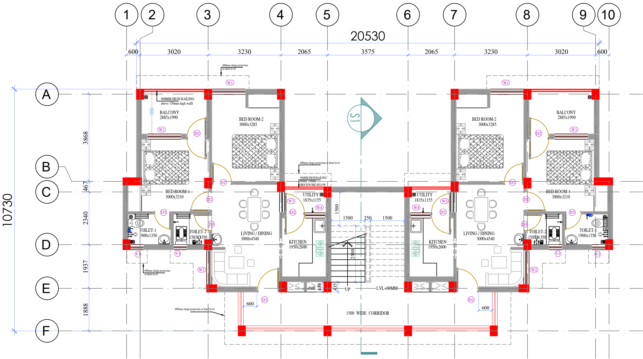
LOWER GROUND FLOOR PLAN.
