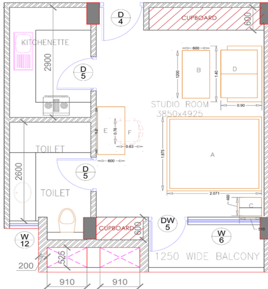
UNIT PLAN - STUDIO ROOM (FURNITURE PLACEMENT) SAI ,NSEC, KOLKATA
