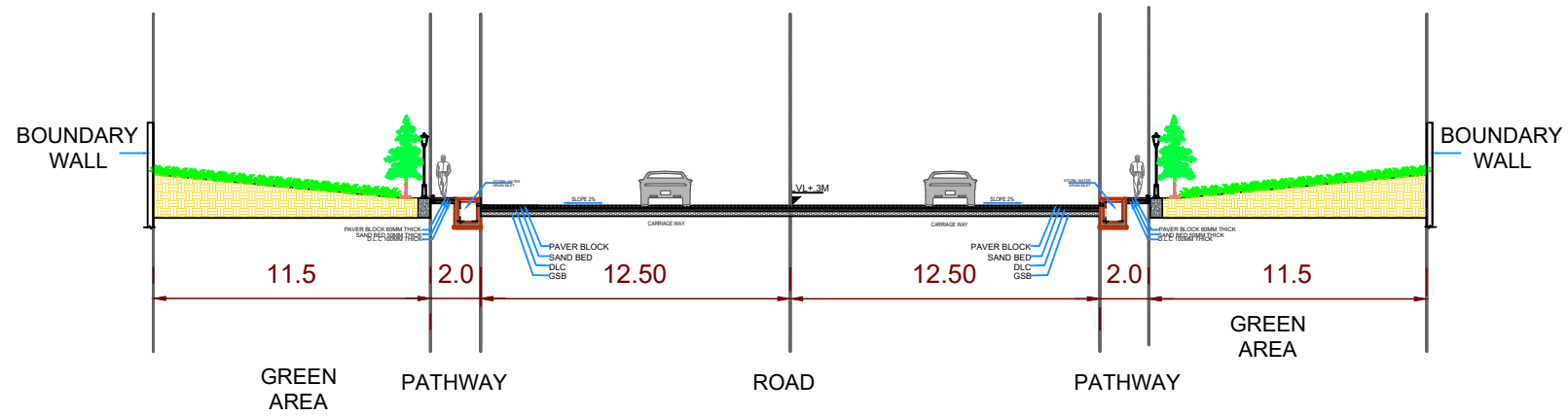
SECTION-AA'
