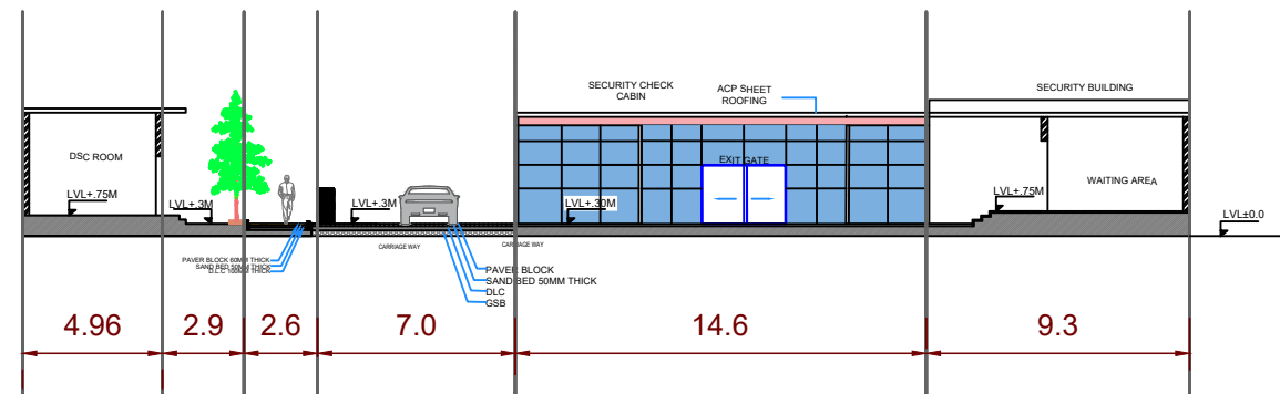
SECTION-XX'
