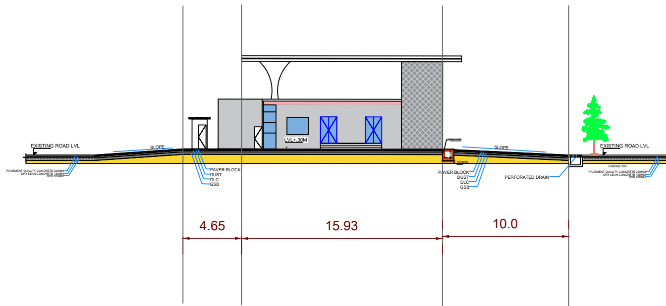
SECTION-YY'
